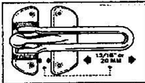
MOUNTING POSITION (with screws provided)
